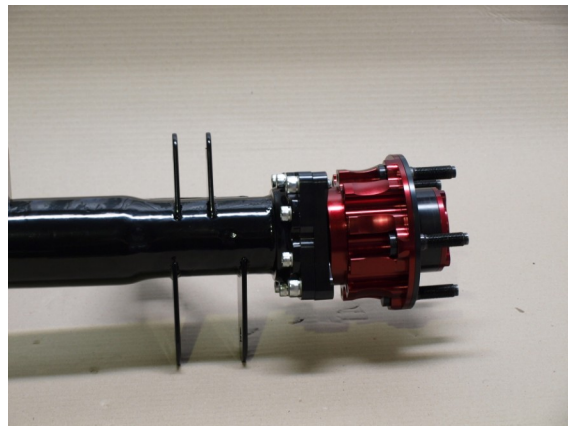
Toe wedges, spindles and fully floating hubs are fitted first
