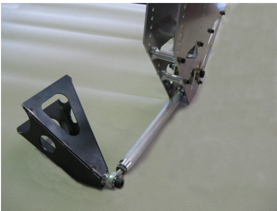
Top quality USA Sourced Rod Ends are used Brackets are CNC drawn, laser cut, and folded for accuracy. Watts Arms Are machined from Billet 6061 Aluminium.
