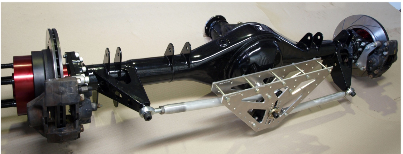
Top quality USA Sourced Rod Ends are used Brackets are CNC drawn, laser cut, and folded for accuracy. Watts Arms Are machined from Billet 6061 Aluminium.
