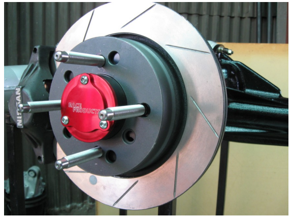
The Fixed Rotor is a 276mm Vented and grooved Rotor, that we machine to suit the application.
